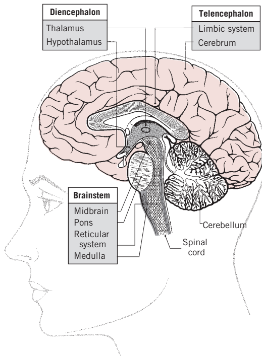
Figure 2-3 A side view of the human brain in cross section, sliced through the middle from front to back. The forebrain, shown shaded in color, consists of the telencephalon (cerebrum and limbic system) and the diencephalon (thalamus and hypothalamus). The remaining divisions of the central nervous system—the cerebellum, the brainstem (shaded gray), and the spinal cord—are also labeled.
