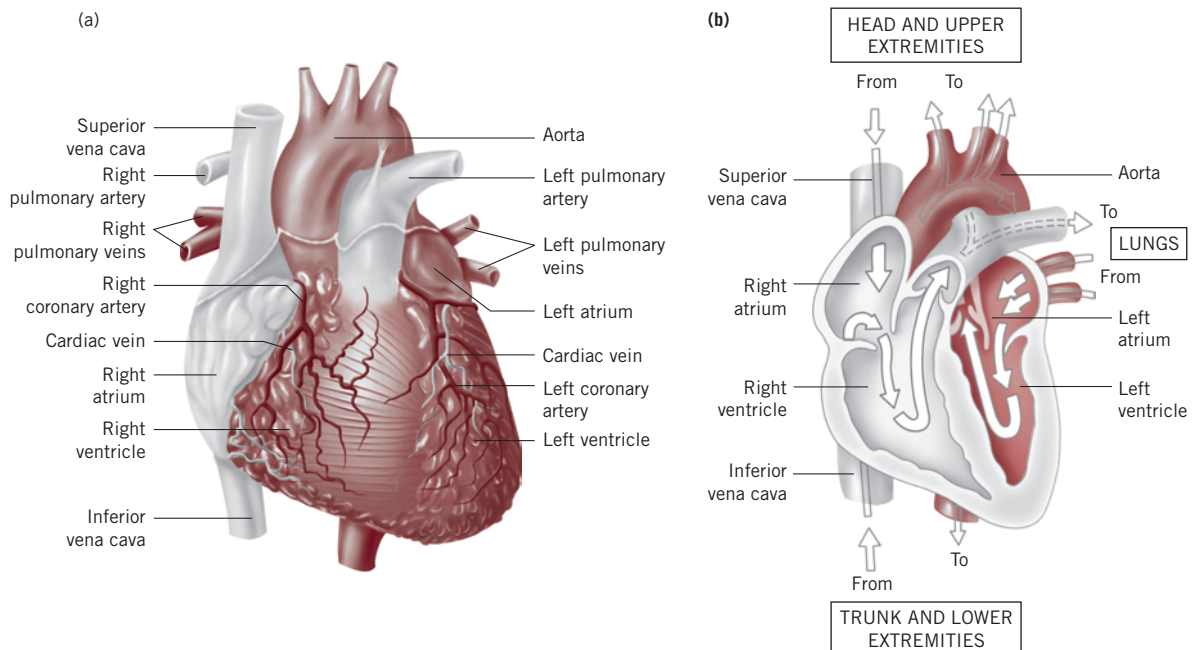
Figure 2-14 Drawings of the heart. (a) An exterior view from the front, showing major blood vessels. The left and right coronary arteries and cardiac veins service the myocardium; larger arteries and veins carry blood to and from the heart's chambers. (b) An interior view of the heart's chambers, showing that blood comes from general circulation—that is, the rest of the body—to the right atrium via the superior and inferior vena cava. The blood then travels to the right ventricle and then to the lungs, where it exchanges \text{CO}_2 for oxygen. The oxygenated blood enters the left atrium via pulmonary veins and goes to the left ventricle , which pumps it via the aorta to the rest of the body.
